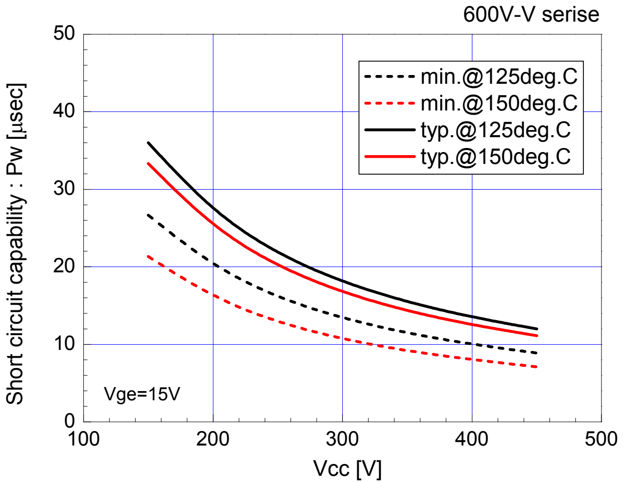
Fig. Relation between applied voltage and short-circuit capacity (600V Family)
