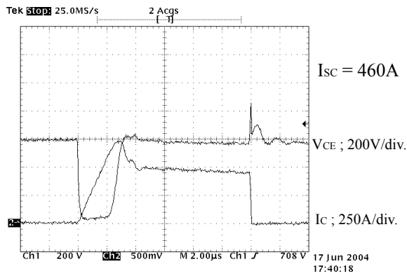
Fig. 4 V GE =13V
