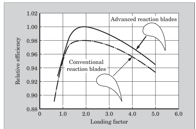
Fig.8 Efficiency of conventional and advanced reaction blades
