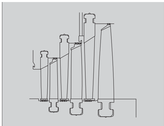
Fig.11 Blading plan for 490 mm low-pressure blades
