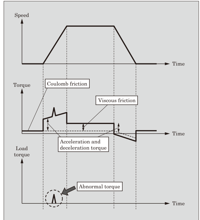
Fig.10 Speed, motor torque and load torque waveforms
