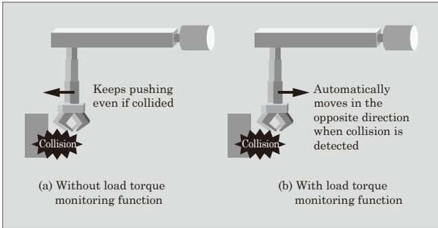
Fig.11 Interference detection by load torque monitoring function
