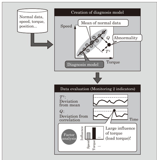
Fig.13 MSPC diagnostic method
