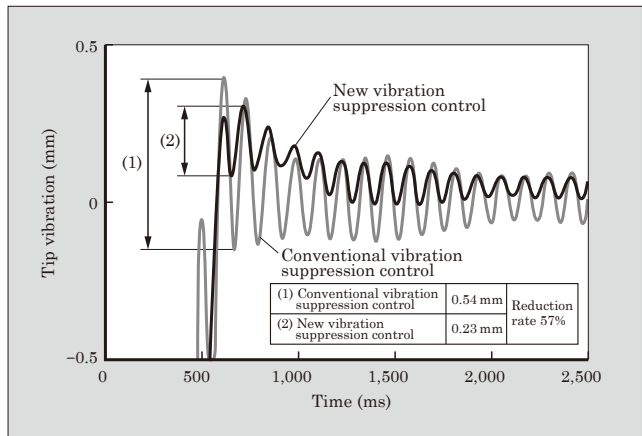
Fig.7 Comparison between waveforms of new and conventional vibration suppression control
