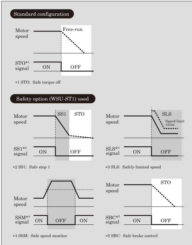
Fig.5 Safety function
