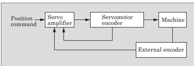
Fig.9 Block diagram of full-closed control of "ALPHA7 Series"
