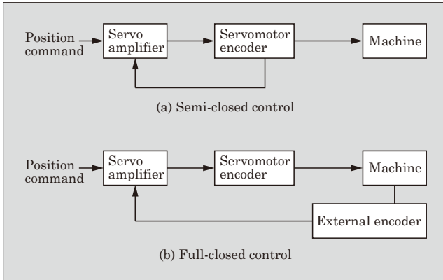
Fig.8 Comparison between block diagrams of semi-closed and full-closed control
