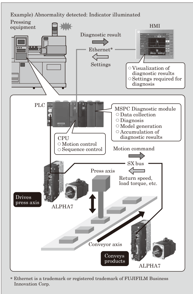
Fig.12 Abnormality detection and diagnosis system combining MSPC
