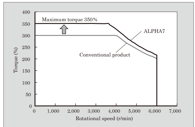
Fig.4 Speed torque characteristics
