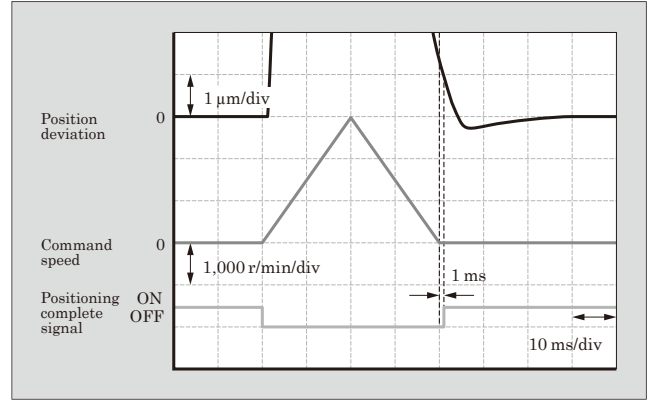
Fig.3 Positioning operation waveforms
