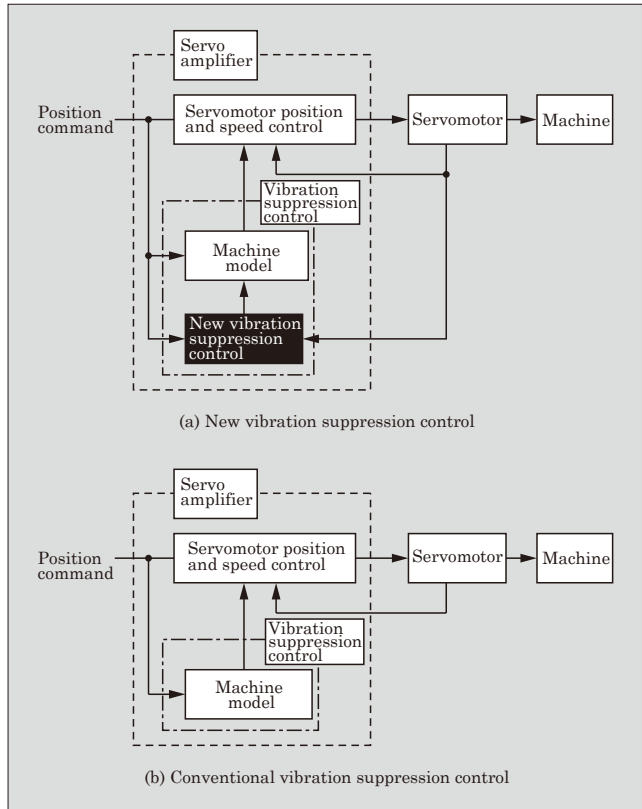
Fig.6 Comparison between block diagrams of new and conventional vibration suppression control
