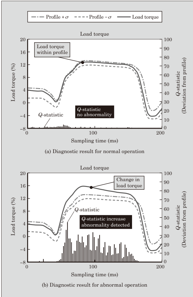
Fig.14 Results of MSPC diagnosis for normal and abnormal data
