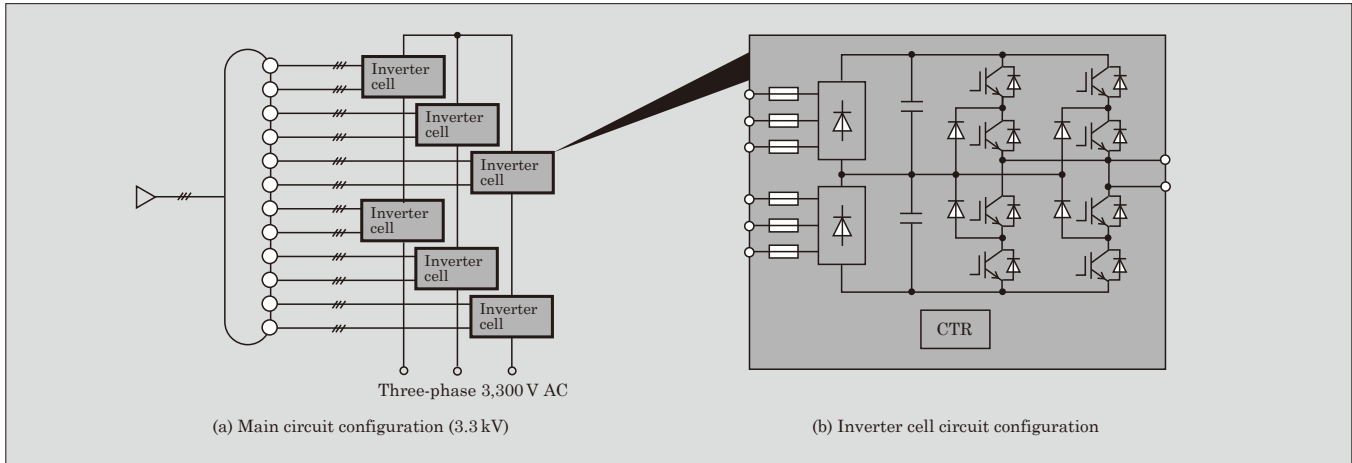
Fig.2 Circuit configuration of medium-voltage inverter
