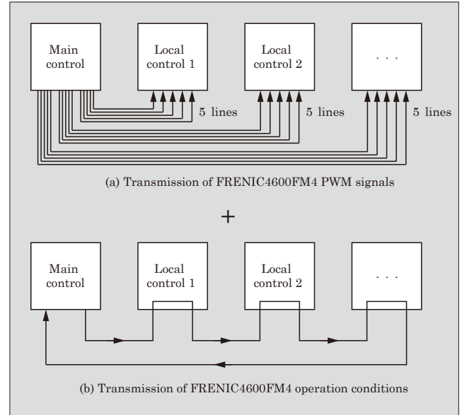
Fig.5 Transmission circuit (conventional)
