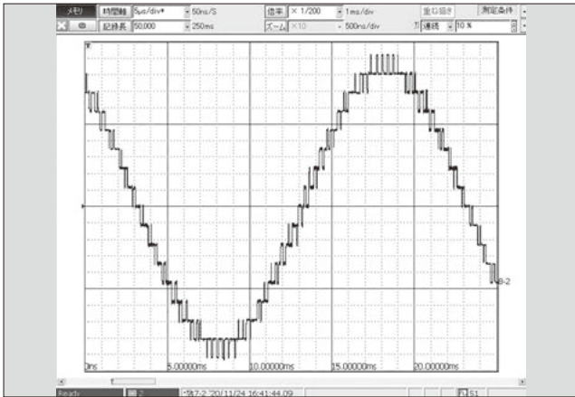
Fig.9 Output voltage waveform during multi-level PWM control (3.3-kV series: between U and V lines)
