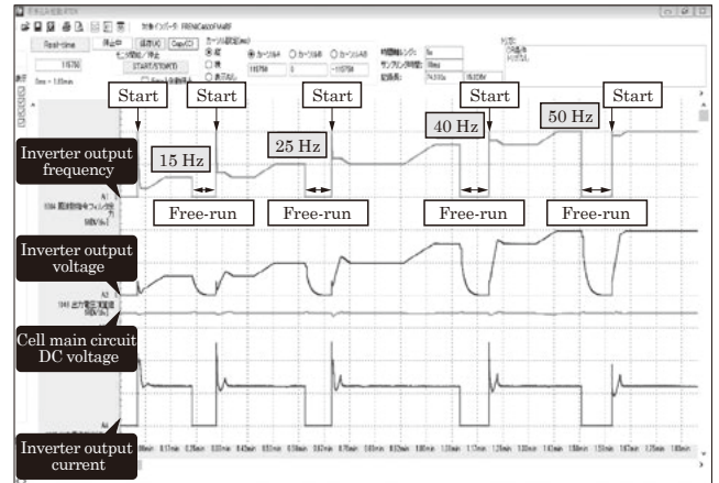
Fig.10 Waveform drawing of free-run restart by chart function
