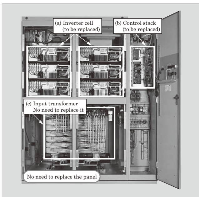
Fig.3 Internal structure of the "FRENIC4600FM4 Series"
