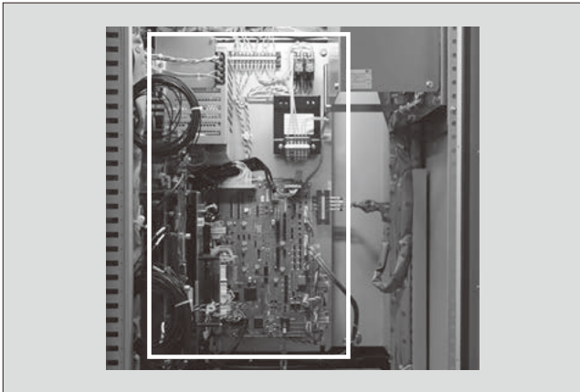
Fig.7 “FRENIC4600FM4RF Series” control stack
