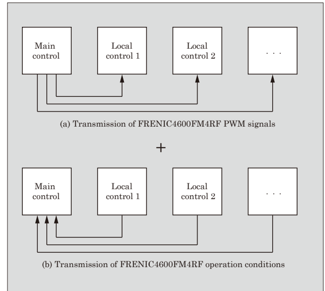
Fig.6 Transmission circuit (retrofit component)
