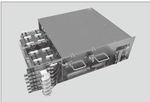
Fig.4 “FRENIC4600FM4RF Series” inverter cell
