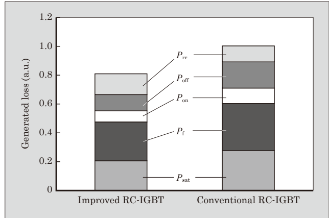
Fig. 11 Loss generated during inverter operation
