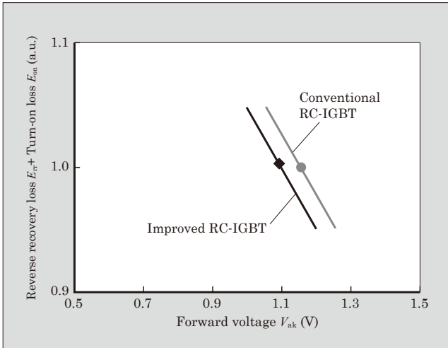
Fig. 10 FWD trade-off characteristics
