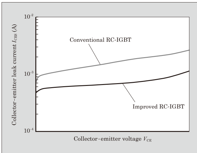
Fig. 6 I_{CES} characteristics ( T_c = 150\text{ }^\circ\text{C} )
