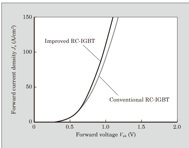
Fig. 7 FWD forward characteristics
