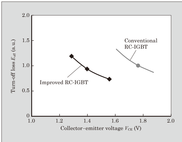
Fig. 5 IGBT trade-off characteristics
