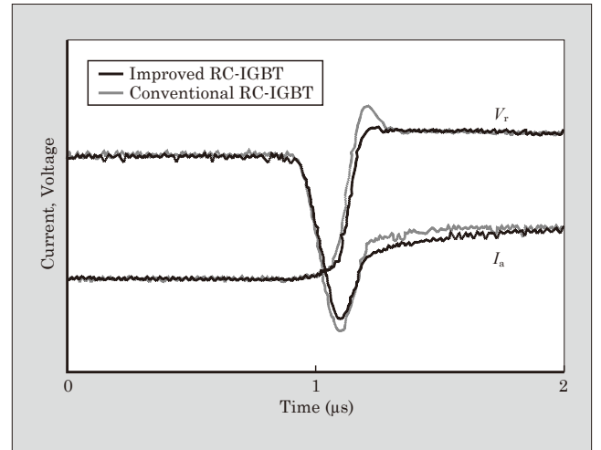
Fig. 8 Switching waveforms during reverse recovery operation
