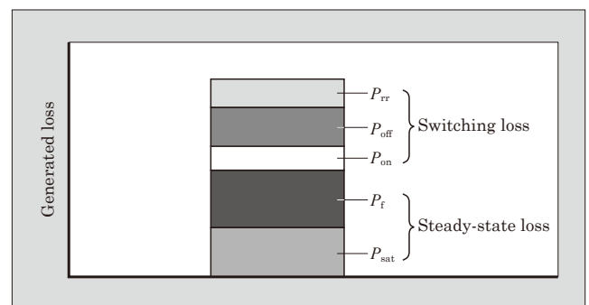
Fig. 2 Example of losses generated in an inverter
