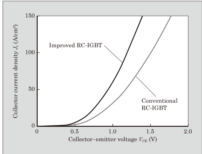
Fig. 3 IGBT Saturation voltage output characteristics
