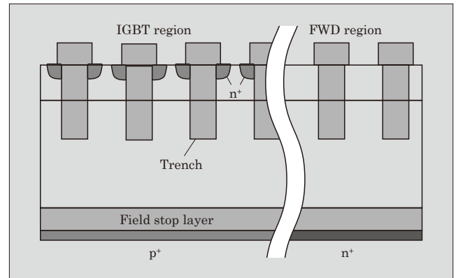
Fig. 1 Schematic structure of an RC-IGBT
