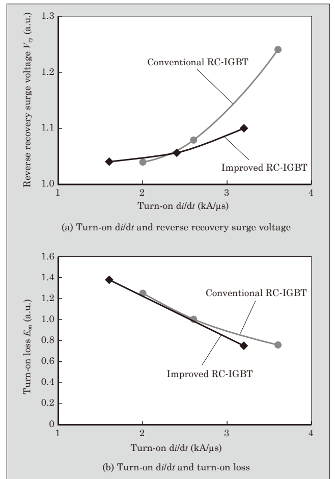
Fig. 9 Characteristics at turn-on
