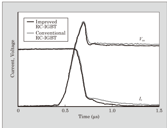
Fig. 4 IGBT turn-off characteristics
