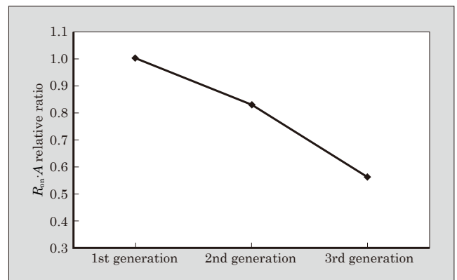
Fig.6 R_{on}\cdot A of trench MOSFETs of respective generations
