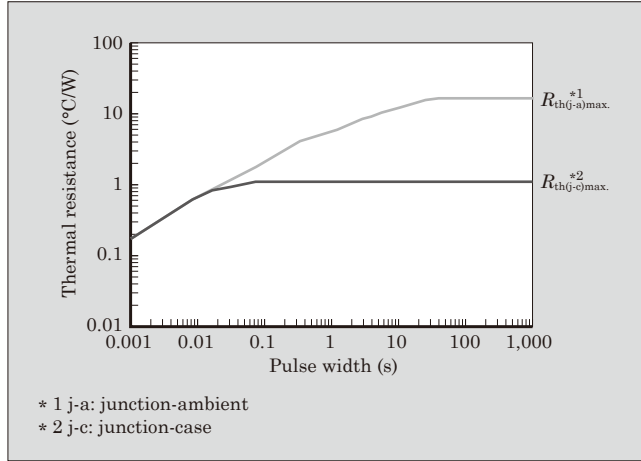
Fig.3 Example of thermal resistance characteristics in board-mounted condition
