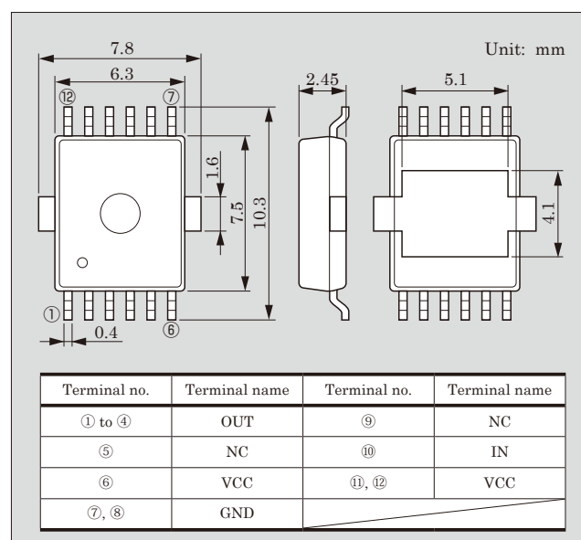
Fig.1 Full view of high-current IPS for vehicles
