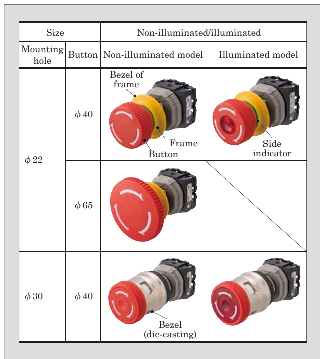
Fig.2 Types of operating element in emergency stop switch
