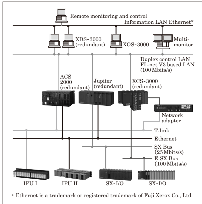
Fig.2 Configuration example for the "MICREX-View XX" system
