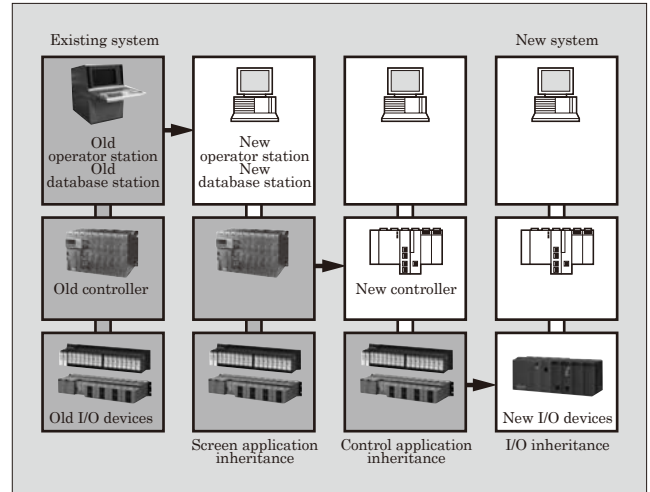
Fig.4 Example of existing system upgrade
