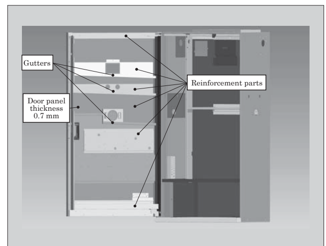
Fig.6 Structure of door panel
