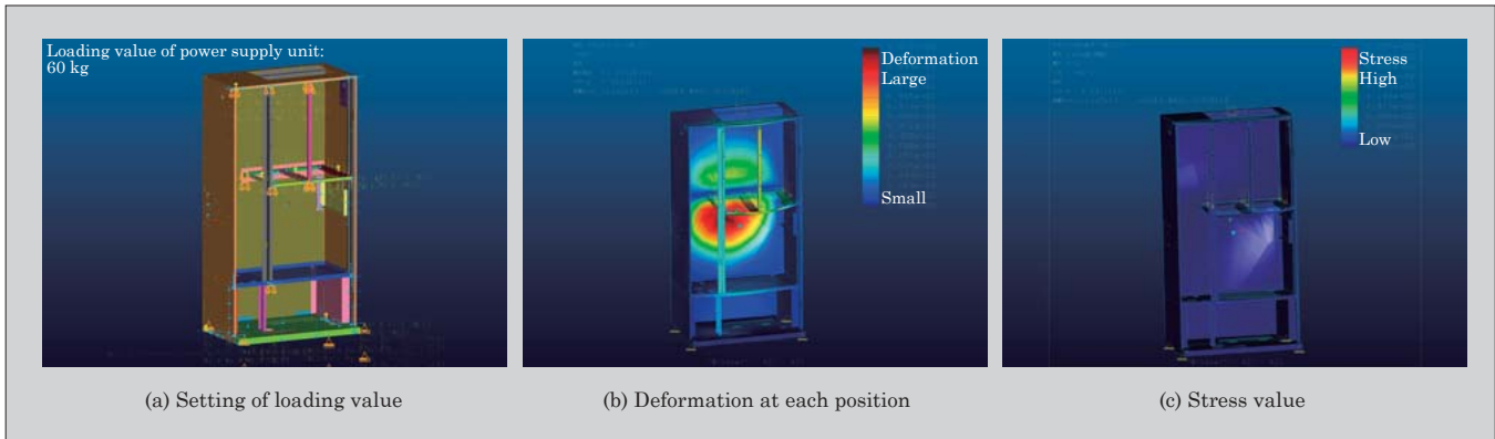
Fig.7 Example of stress analysis
