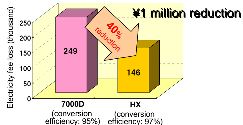
Electricity fee loss of high-efficiency UPSs (load power factor: 0.9)
